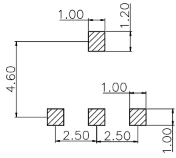
PCB Layout
